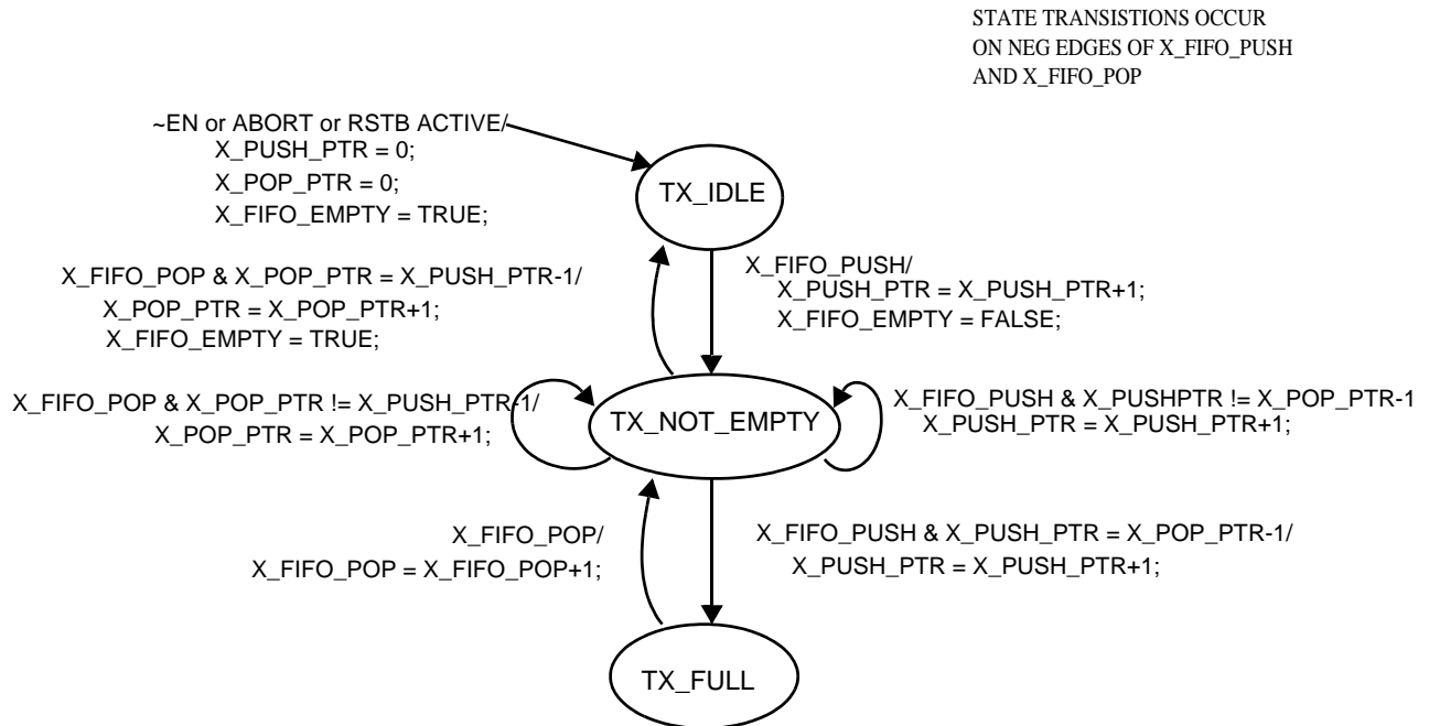
Figure 22. State Diagram of Transmit FIFO
