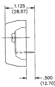
“Y” Terminals
