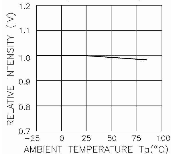
Relative Intensity vs. Ambient Temperature
