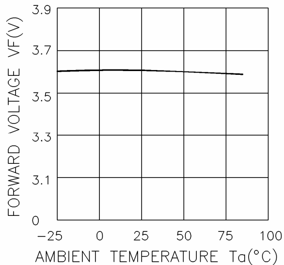
Forward VoUTage vs. Ambient Temperature
