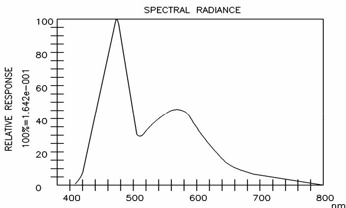
Luminous Spectrum (Ta=25°C)
