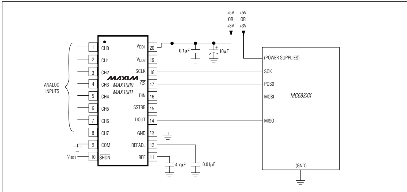
Figure 17. QSPI Connections
