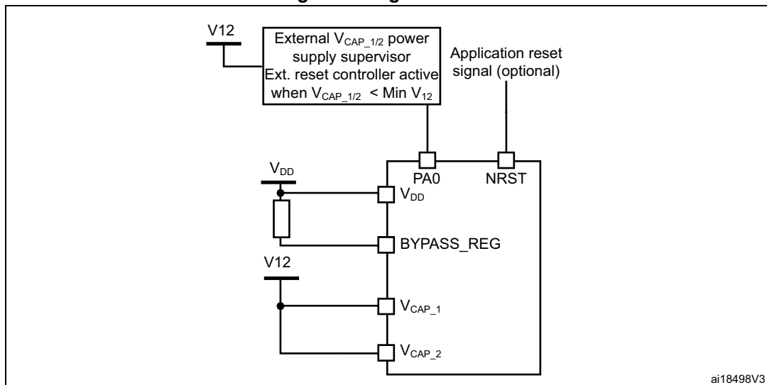
Figure 8. Regulator OFF
