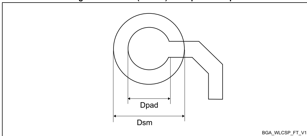
Figure 90. UFBGA(176+25) - Footprint example
