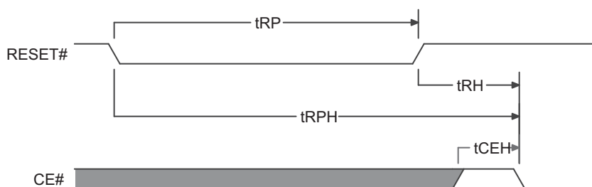
Figure 10.4 Hardware Reset
