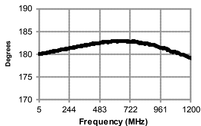
Phase Balance
