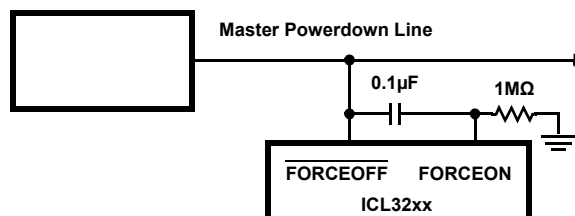
Figure 12. Circuit to Ensure Immediate Power Up When Exiting Forced Powerdown
