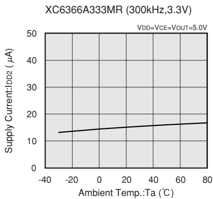
(8) SUPPLY CURRENT 2 vs. AMBIENT TEMPERATURE
