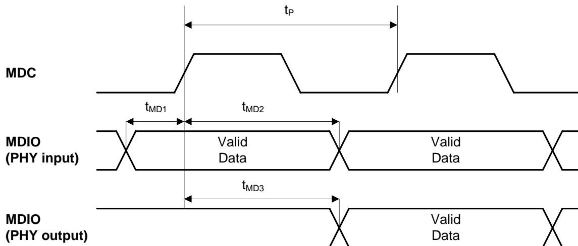
Figure 19. MDC/MDIO Timing
