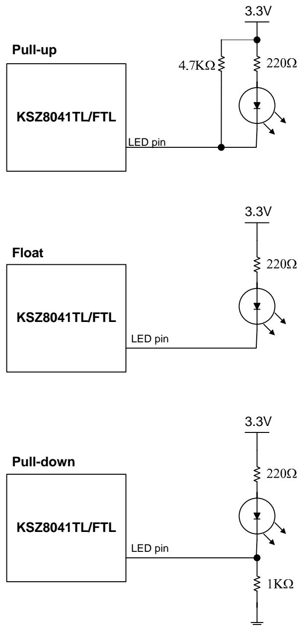
Figure 23. Reference Circuits for LED Strapping Pins
