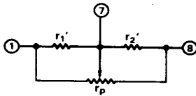
Figure 1. High Resolution, High Stability Nulling Circuit
