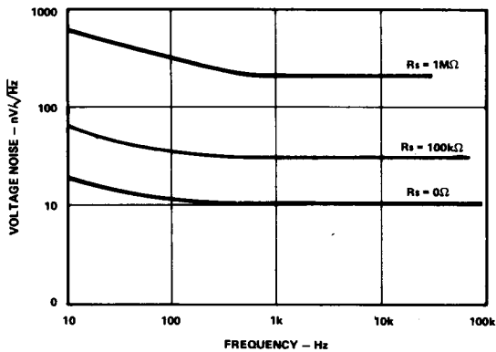
Figure 7. Voltage Noise vs. Frequency
