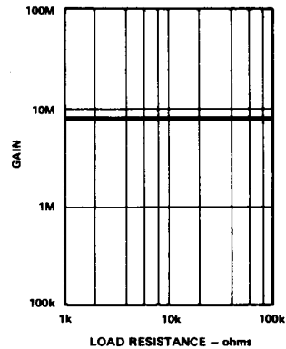
Figure 6. Gain vs. Load Resistance
