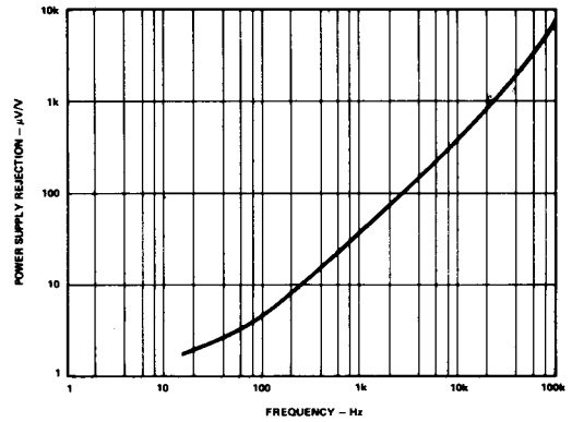
Figure 4. PSRR vs. Frequency
