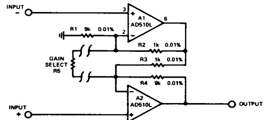
Figure 2. Instrumentation Amplifier
