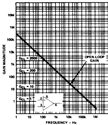
Figure 3. Small Signal Gain vs. Frequency
