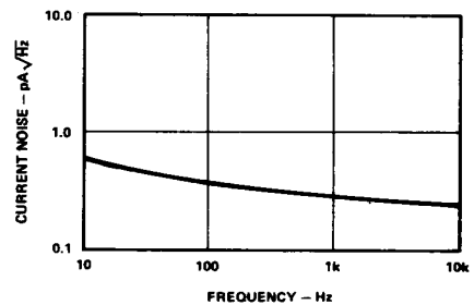
Figure 8. Current Noise vs. Frequency
