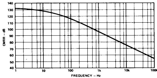
Figure 5. CMRR vs. Frequency
