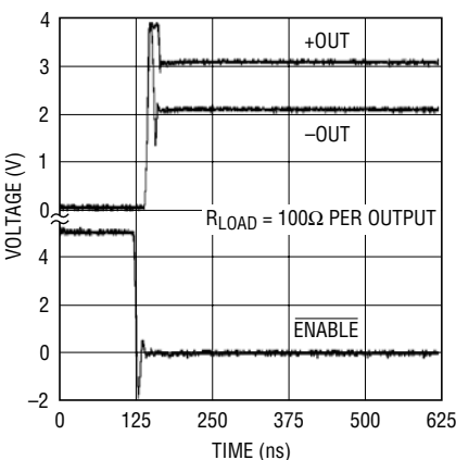
Turn-On Time
