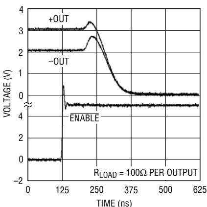
Turn-Off Time
