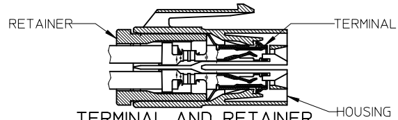
TERMINAL AND RETAINER ASSEMBLY DRAWING
