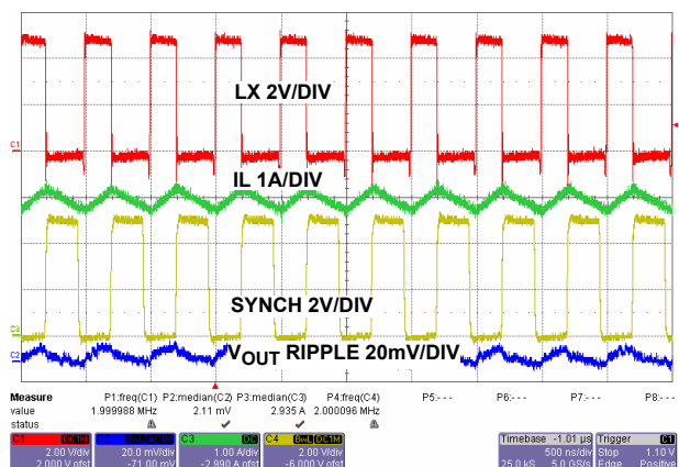
FIGURE 29. STEADY STATE OPERATION AT FULL LOAD WITH FREQUENCY = 2MHz
