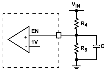
FIGURE 37. EXTERNAL RESISTOR DIVIDER
