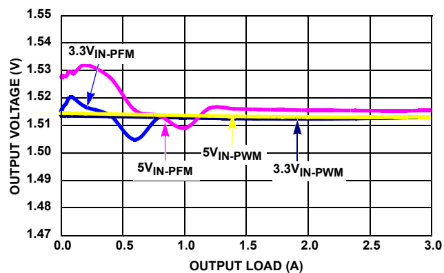
FIGURE 10. V_{OUT} REGULATION vs LOAD (1MHz, V_{OUT} = 1.5\text{V} )
