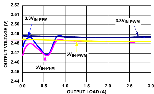
FIGURE 12. V_{OUT} REGULATION vs LOAD (1MHz, V_{OUT} = 2.5\text{V} )
