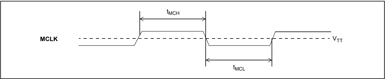
Figure 14 - Master Clock
