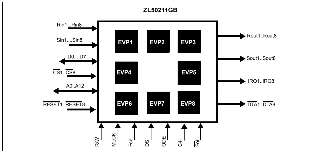
Figure 1 - ZL50211 Device Overview
