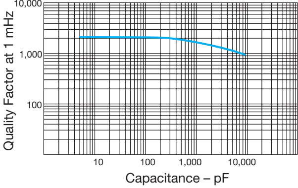
Quality Factor vs. Capacitance Axial
