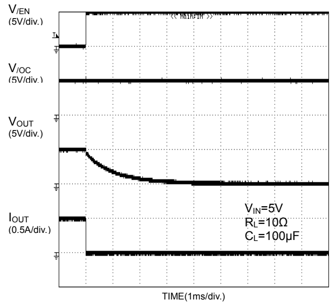
Figure 29. Output Fall Characteristic (BD2061AFJ)
