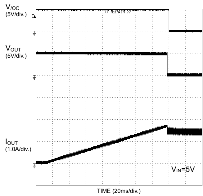
Figure 31. Over Current Response Ramped Load (BD2061AFJ)
