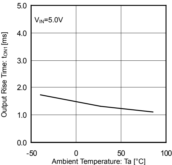
Figure 19. Output Rise Time vs Ambient Temperature
