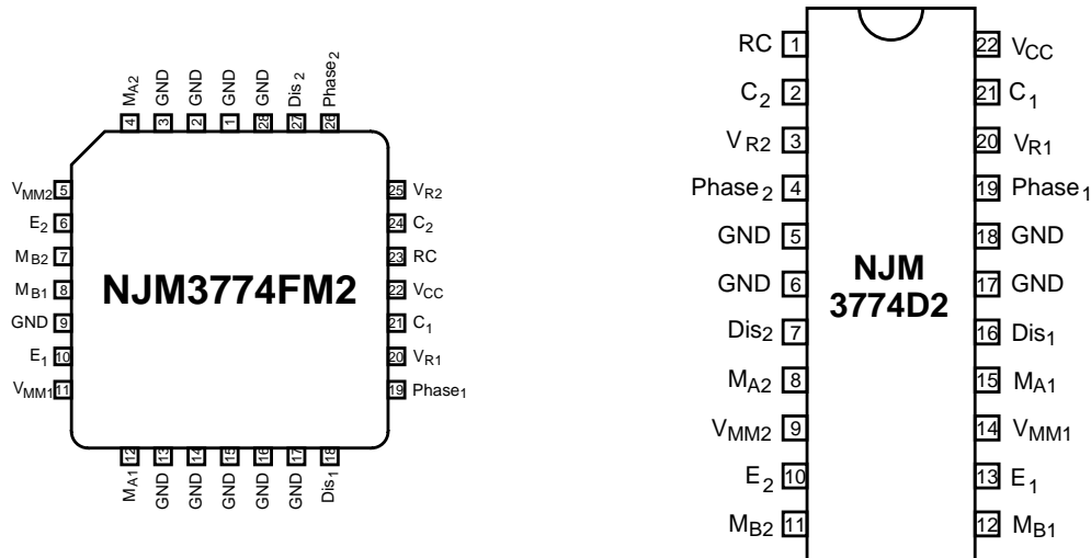
Figure 2. Pin configurations
