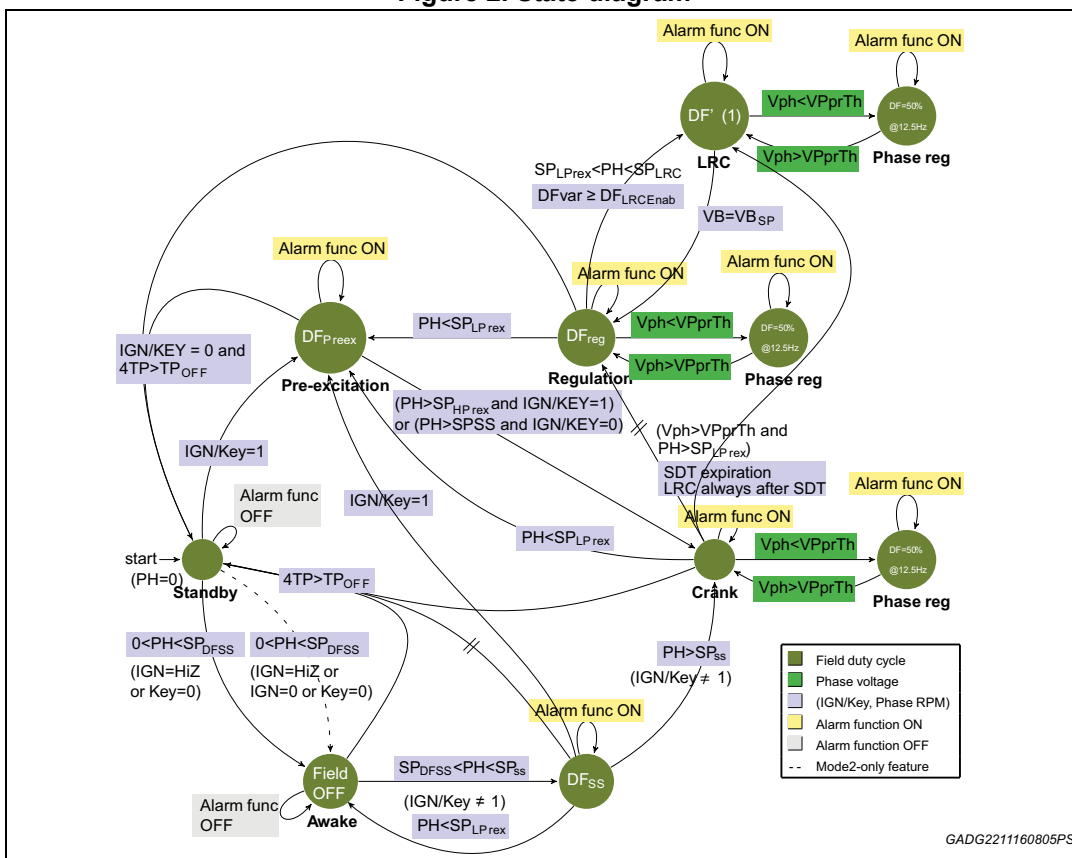
Figure 2. State diagram
