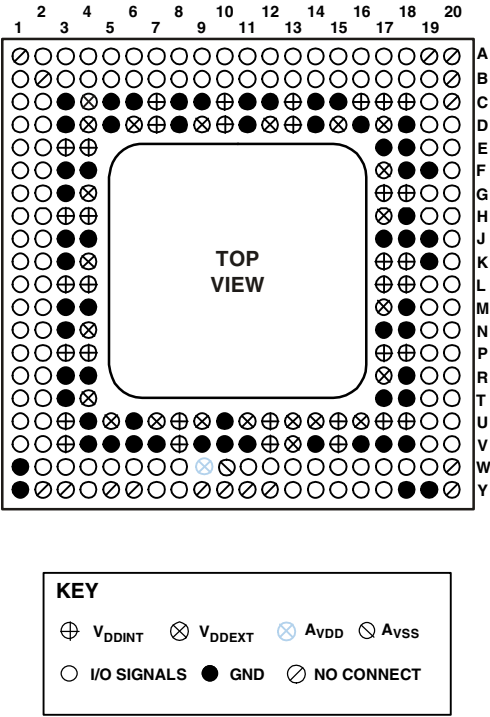
Figure 50. 256-Ball BGA_ED Ball Configuration (Top View)
