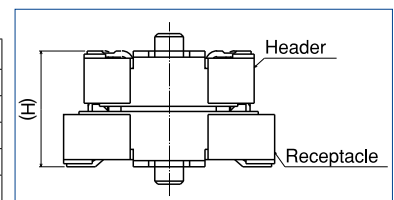
(H):Reference dimension
