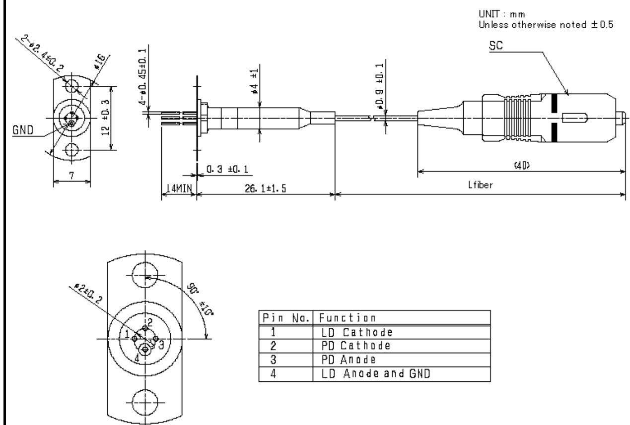
FU-450SDF-FW1M2
