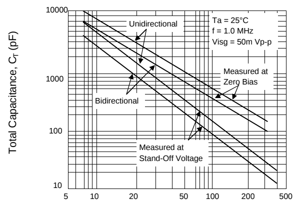
FIG.5 - TOTAL CAPACITANCE
