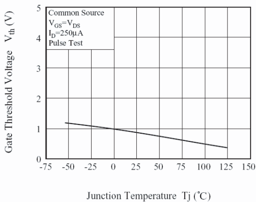
Fig5. V_{th} - T_j
