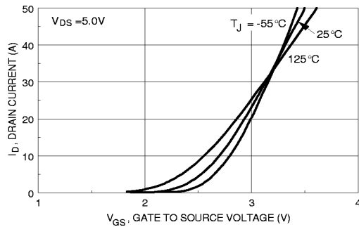
Figure 5. Transfer Characteristics.
