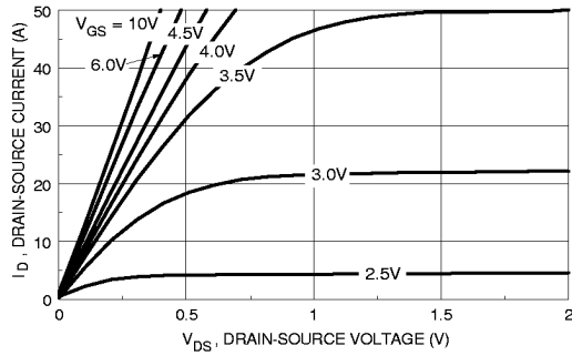
Figure 1. On-Region Characteristics.
