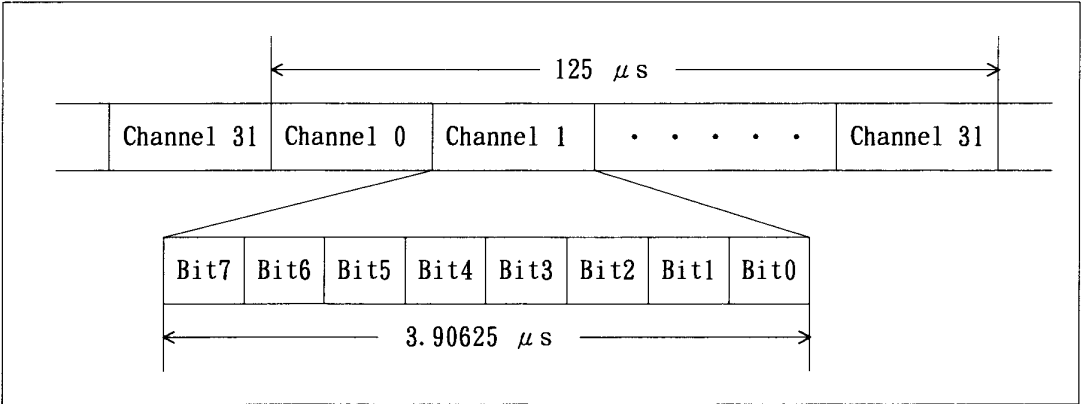
Fig-7 PCM-BUS Stream Format Diagram
