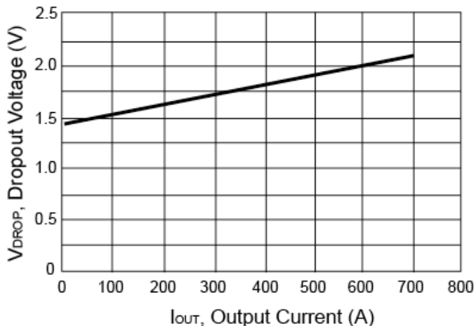
Figure 4. V_{drop} vs. Output Current
