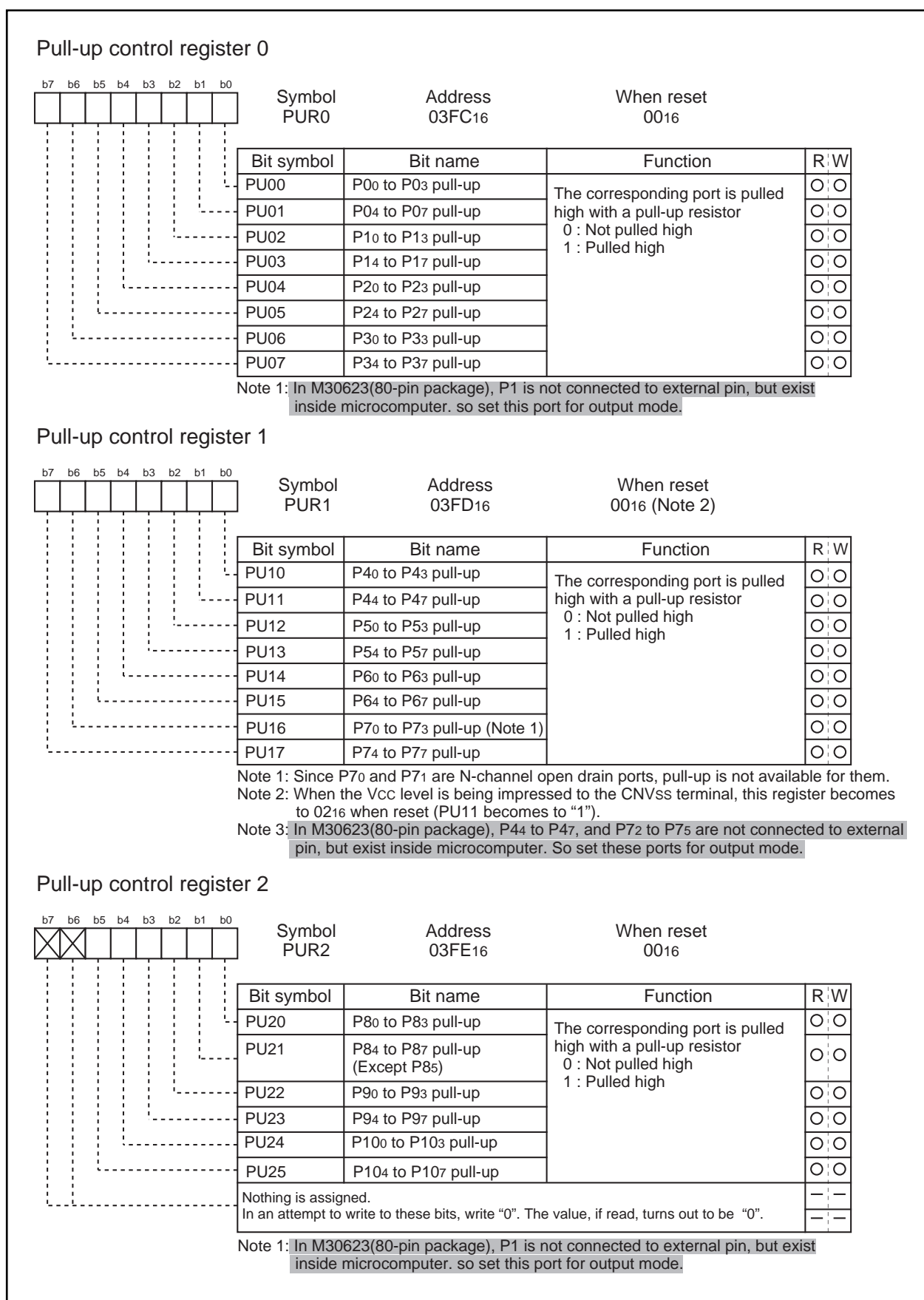
Figure 1.23.7. Pull-up control register
