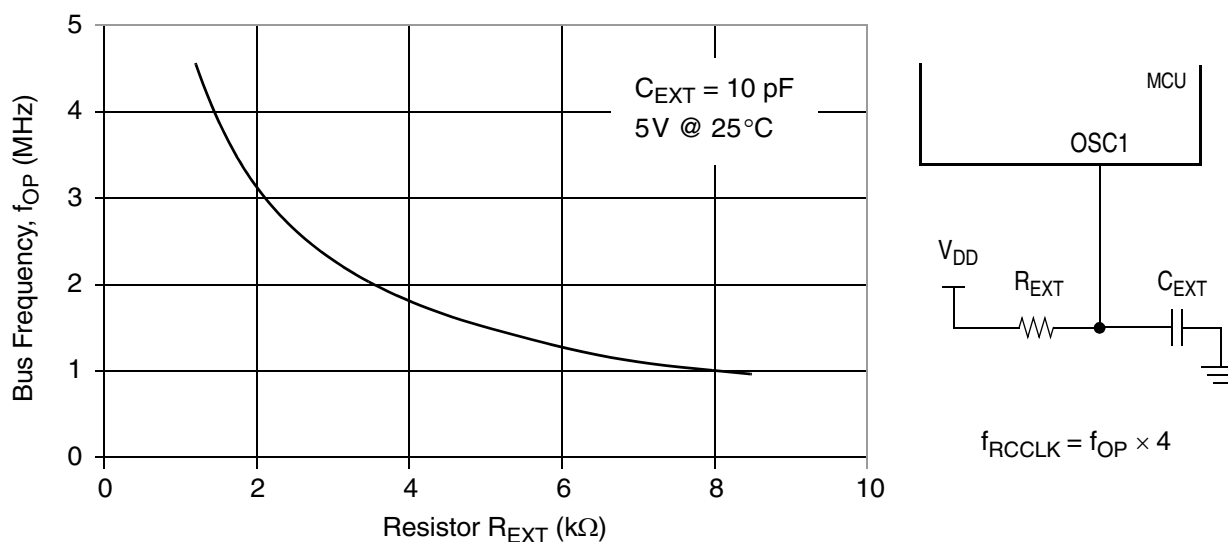
Figure 24-1. RC vs. Bus Frequency (5V @ 25°C)
