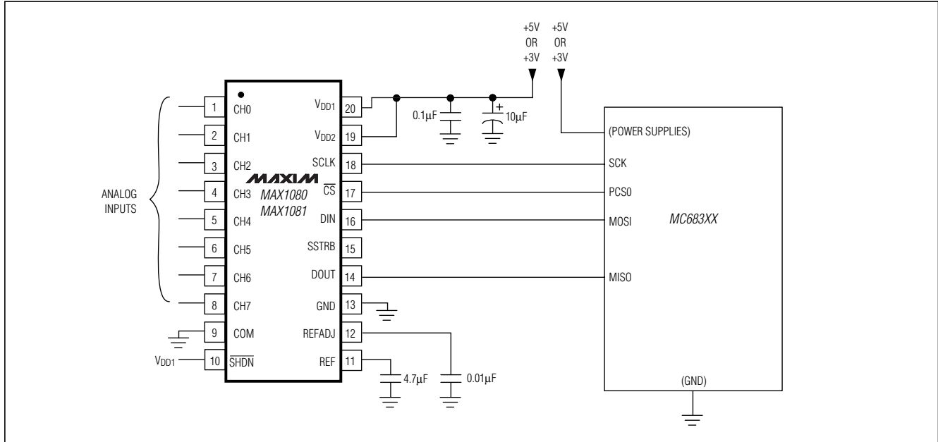
Figure 17. QSPI Connections
