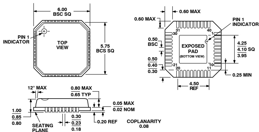
COMPLIANT TO JEDEC STANDARDS MO-220-VJJD-2 Figure 20. 40-Lead Lead Frame Chip Scale Package [LFCSP_VQ] 6 mm × 6 mm Body, Very Thin Quad (CP-40) Dimensions shown in millimeters
