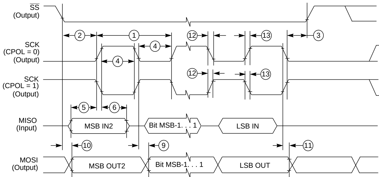
Figure A-8. SPI Master Timing (CPHA = 0)
