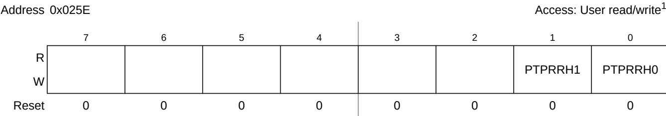
Figure 2-35. Port P Routing Register High (PTPRRH)
