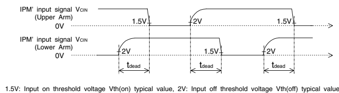
Fig. 7 Dead time measurement point example
