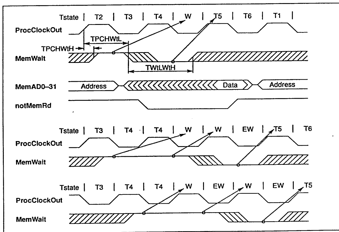
Figure 7.16 IMS T425 memory wait timing
