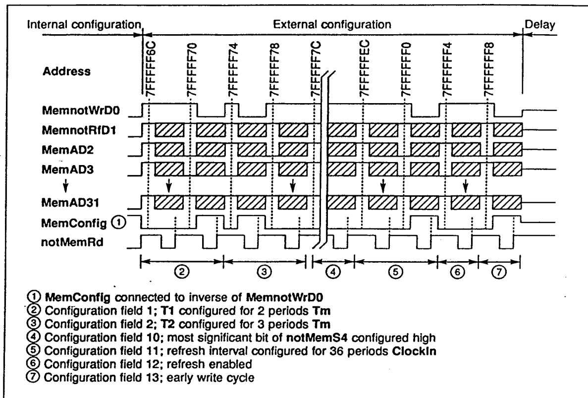
Figure 7.12 IMS T425 external configuration scan
