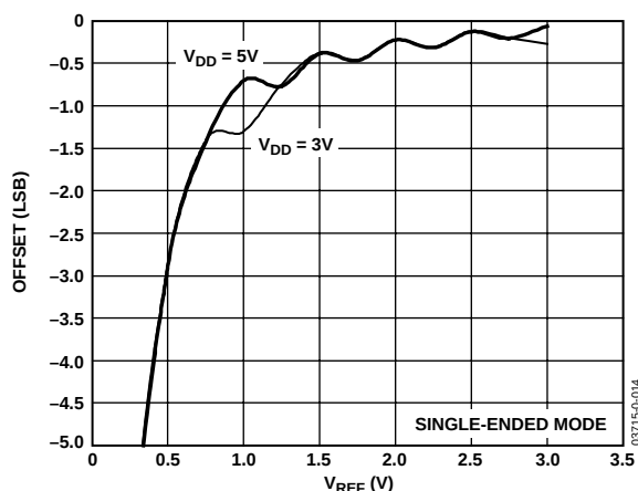
Figure 11. AD7938 Offset vs. V_{REF}
