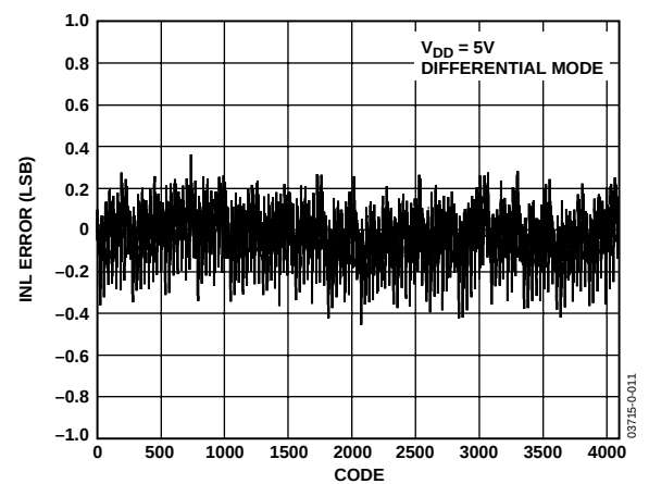
Figure 8. AD7938 Typical INL @ V_{DD} = 5\text{V}
