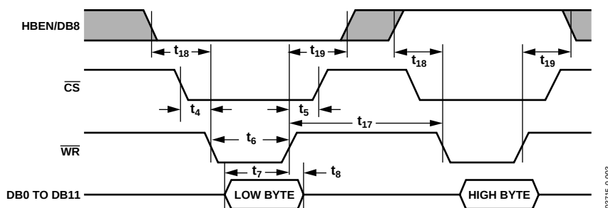
Figure 38. AD7938/AD7939 Parallel Interface—Write Cycle Timing for Byte Mode Operation ( \overline{W}/\overline{B} = 0 )
