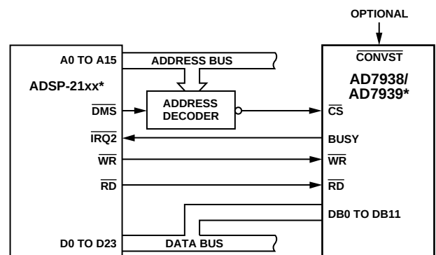
Figure 42. Interfacing to the ADSP-21xx
