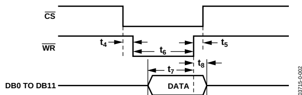
Figure 37. AD7938/AD7939 Parallel Interface—Write Cycle Timing for Word Mode Operation ( \overline{W}/\overline{B} = 1 )
