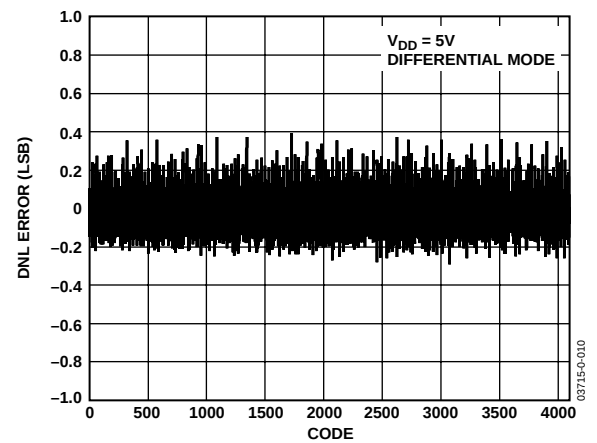
Figure 7. AD7938 Typical DNL @ V_{DD} = 5\text{V}
