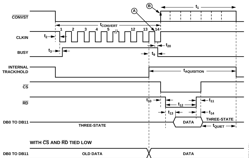
Figure 35. AD7938/AD7939 Parallel Interface—Conversion and Read Cycle in Word Mode ( \overline{W/B} = 1 )
