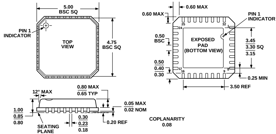
Figure 46. 32-Lead Lead Frame Chip Scale Package [LFCSP] 5 mm × 5 mm Body (CP-32-3) Dimensions shown in millimeters
