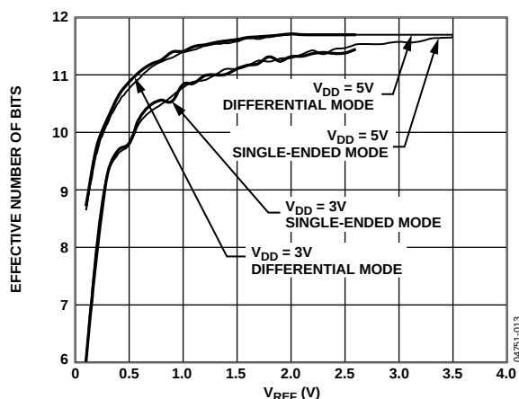
Figure 10. AD7938 ENOB vs. V_{REF}
