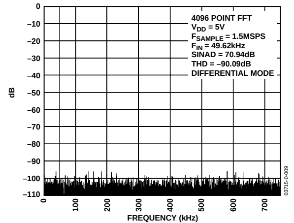
Figure 6. AD7938 FFT @ V_{DD} = 5\text{V}
