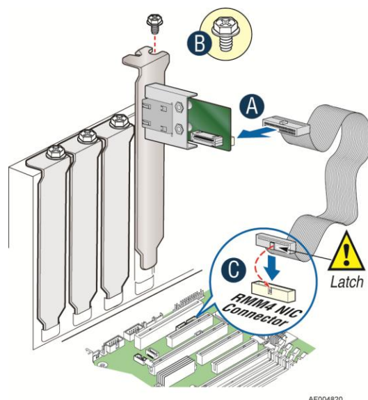
Figure 23. Intel® RMM4 Dedicated Management NIC Installation
