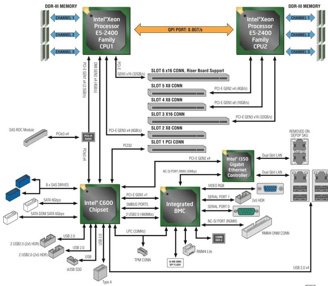
Figure 13. Intel® Server Board S2400GP Functional Block Diagram
