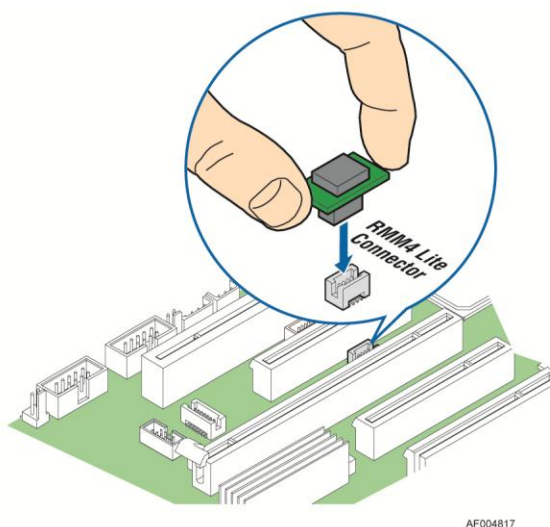
Figure 22. Intel® RMM4 Lite Activation Key Installation
