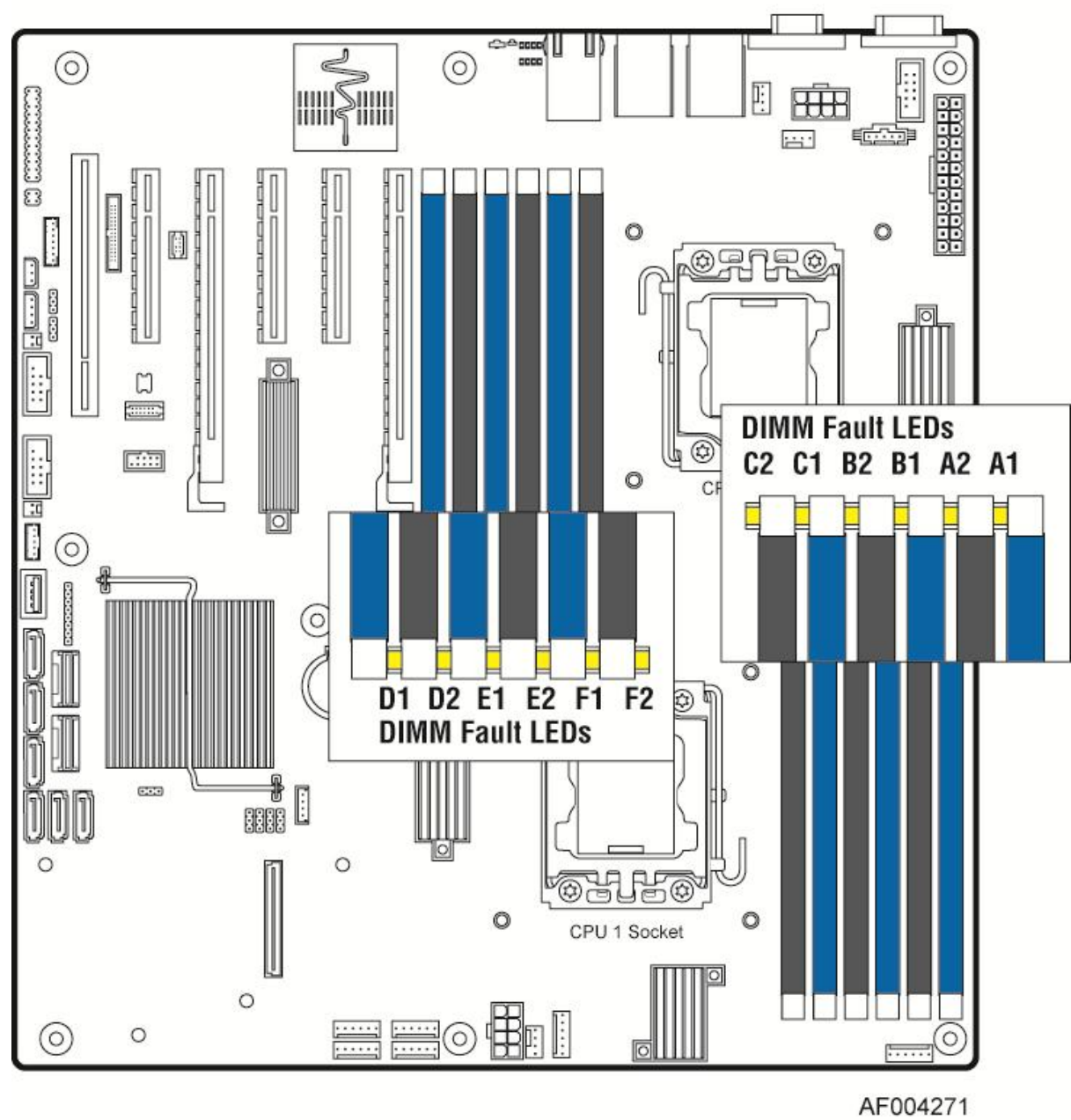
Figure 29. DIMM Fault LEDs Location
