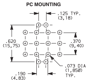
8421SD3V4GE 4PDT
