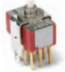
8421SD3V4GE 4PDT
