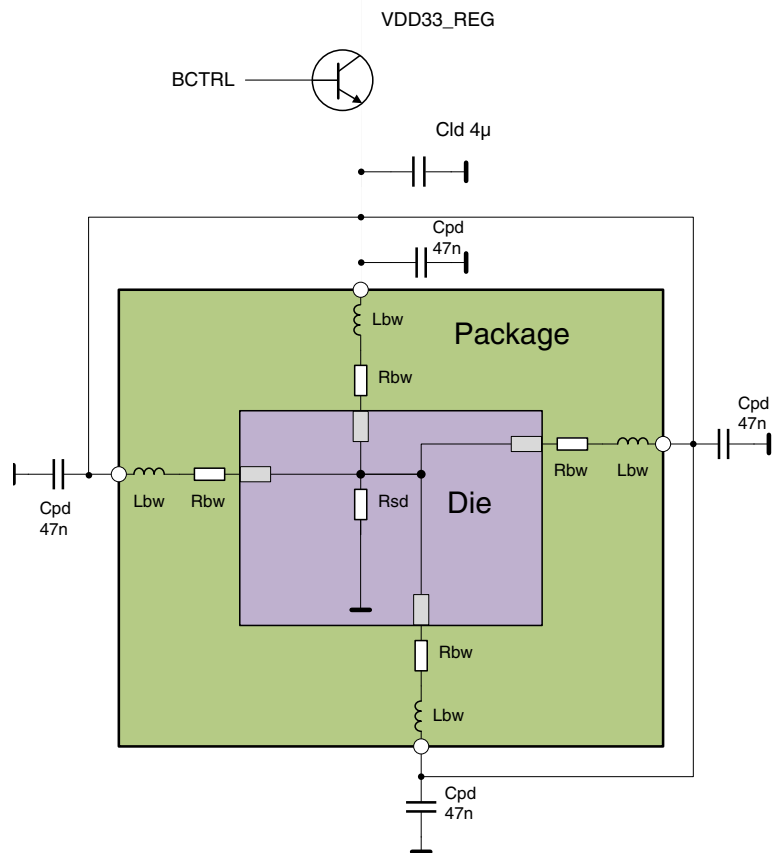
Figure 4. Core supply decoupling and parasitics
