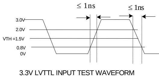
Figure 5. 3.3V LVTTTL and 2.5V LVTTTL Input Test Waveforms
