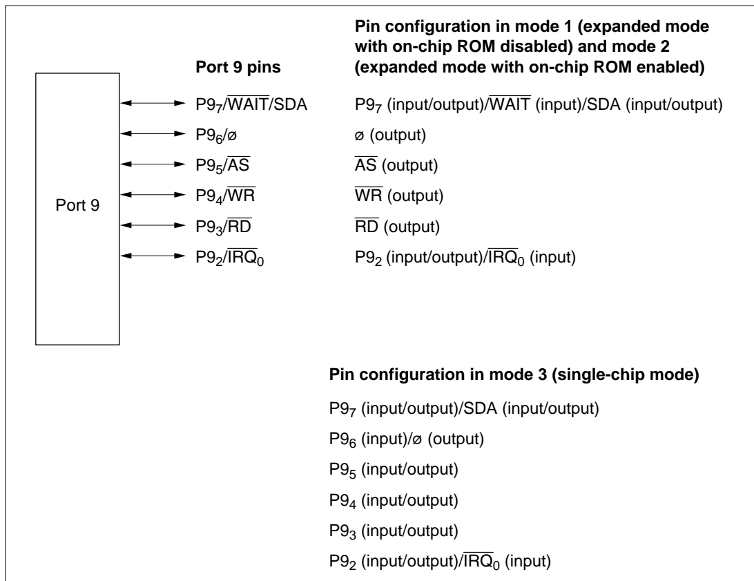
Figure 7.17 Port 9 Pin Configuration
