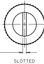
SLOTTED
