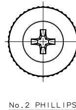
No. 2 PHILLIPS
