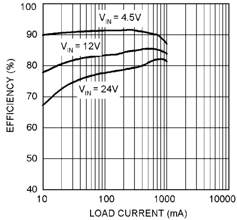
Efficiency vs Load Current ( V_{OUT} = 3.3V , L = 22\mu H )
