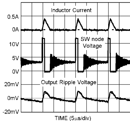
Discontinuous Mode Operation (V_{IN} = 12V, V_{OUT} = 3.3V, I_{OUT} = 50mA, L = 22\mu H)
