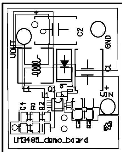
Silk Screen
