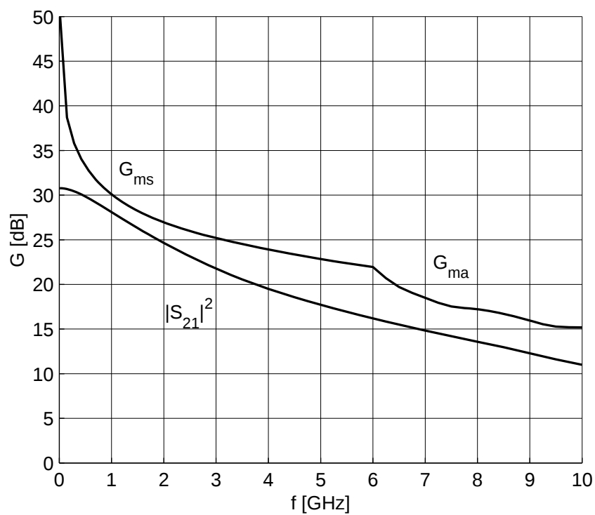
Figure 5-10 Gain G_{ma} , G_{ms} , |S_{21}|^2 = f(f) , V_{CE} = 3 V, I_C = 15 mA
