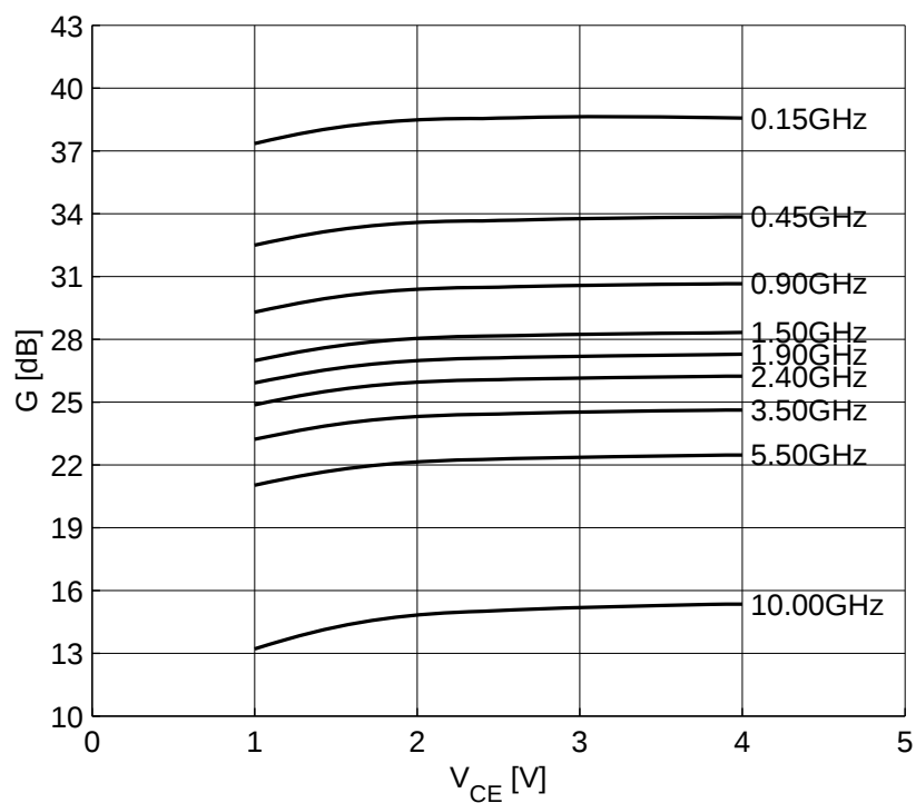
Figure 5-12 Maximum Power Gain G_{\max} = f(V_{CE}) , I_C = 15 \text{ mA} , f = \text{Parameter in GHz}
