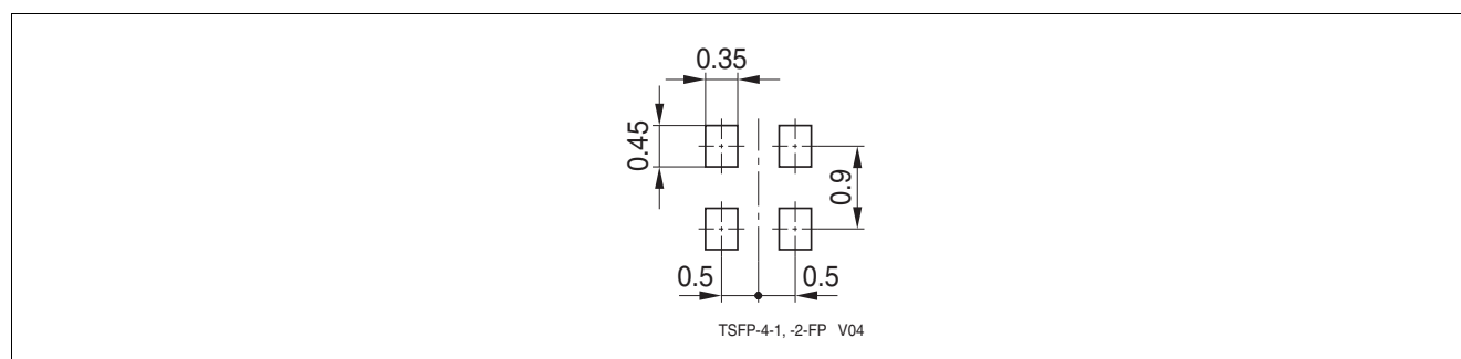
Figure 7-2 Package Footprint
