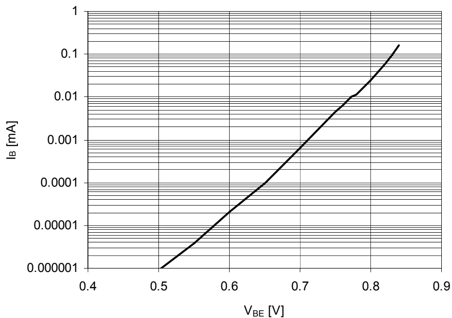
Figure 5-5 Base Current vs. Base Emitter Forward Voltage I_B = f(V_{BE}) , V_{CE} = 2\text{ V}
