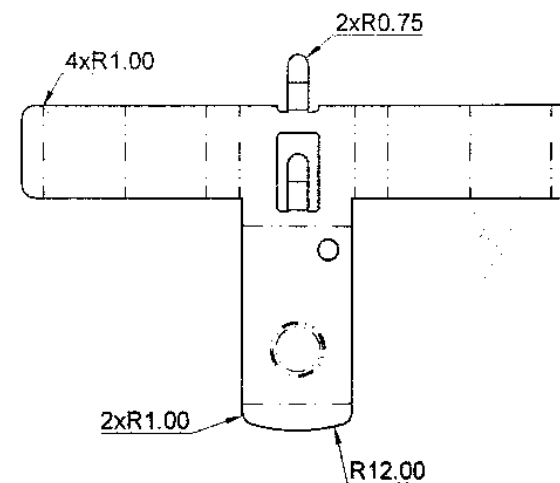
UNBEND VIEW
