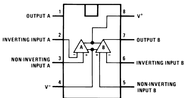
Dual-In-Line Package
