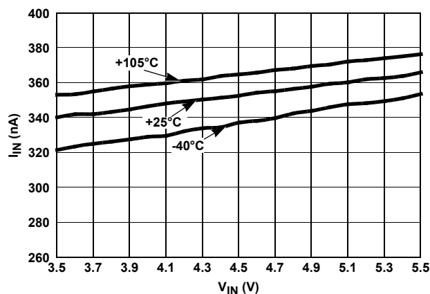
FIGURE 99. I_{IN} vs V_{IN} OVER-TEMPERATURE
