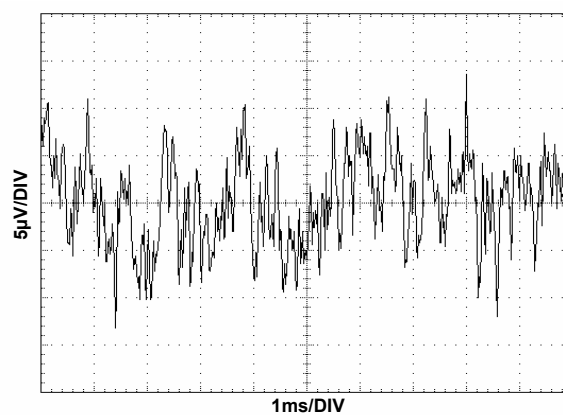
FIGURE 55. V_{OUT} NOISE
