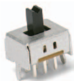
OS202011MS2QS1 DPDT
