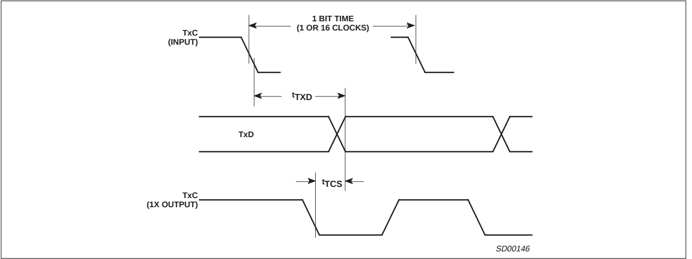
Figure 10. Transit Timing
