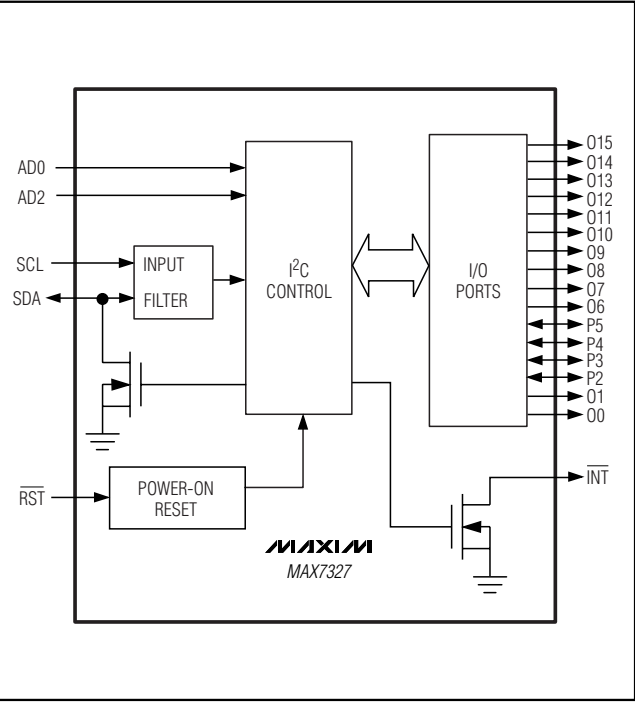
Functional Diagram
