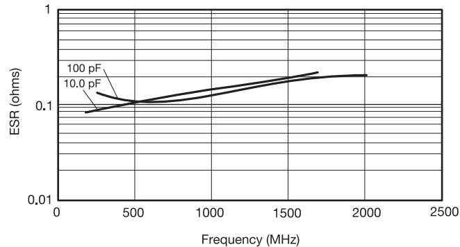
TYPICAL ESR vs. FREQUENCY 0805 “U” SERIES
